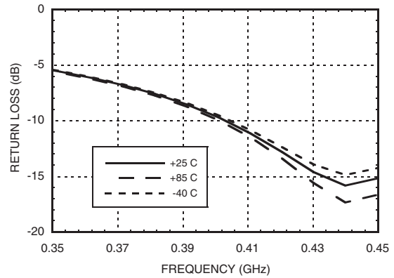
Output Return Loss vs. Temperature @ 400 MHz
