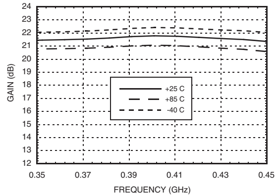
Gain vs. Temperature @ 400 MHz
