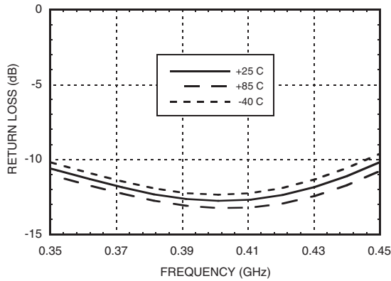
Input Return Loss vs. Temperature @ 400 MHz
