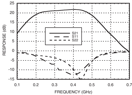
Broadband Gain & Return Loss @ 400 MHz
