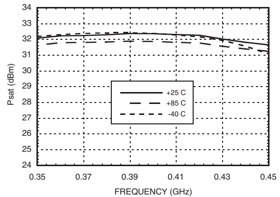
Psat vs. Temperature @ 400 MHz
