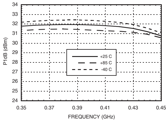
P1dB vs. Temperature @ 400 MHz
