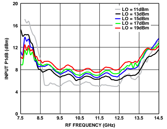
Figure 17. Input P1dB vs. RF Frequency at Various LO Power Levels, TA = 25°C
