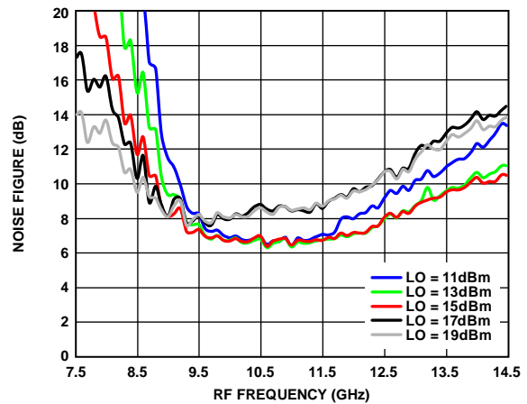
Figure 18. Noise Figure vs. RF Frequency at Various LO Power Levels, TA = 25°C
