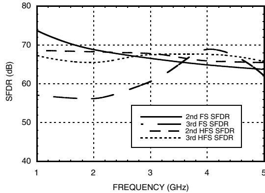
Hold-Mode SFDR vs. Frequency & Input Power @ f_{clk} = 500 \text{ MHz} @ +10 \text{ dBm}
