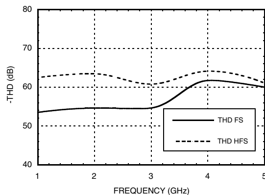
Hold-Mode THD vs. Frequency & Input Power @ f_{clk} = 2 \text{ GHz} @ 0 \text{ dBm}
