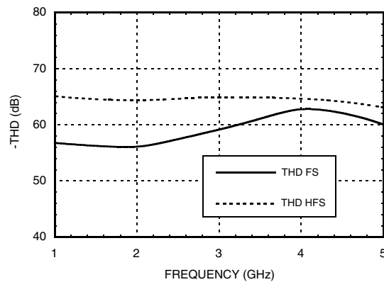
Hold-Mode THD vs. Frequency & Input Power @ f_{clk} = 1 \text{ GHz} @ +6 \text{ dBm}
