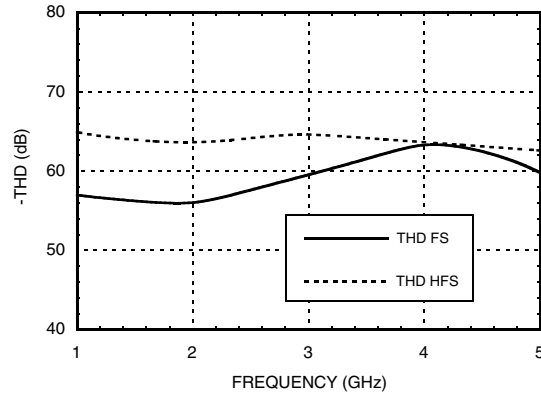
Hold-Mode THD vs. Frequency & Input Power @ f_{clk} = 500 \text{ MHz} @ +10 \text{ dBm}
