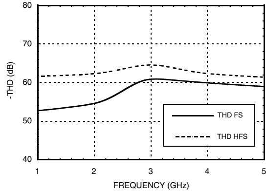
Hold-Mode THD vs. Frequency & Input Power @ f_{clk} = 3 \text{ GHz} @ 0 \text{ dBm}
