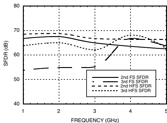
Hold-Mode SFDR vs. Frequency & Input Power @ f_{clk} = 2 \text{ GHz} @ 0 \text{ dBm}
