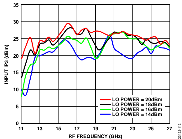
Figure 112. Input IP3 vs. RF Frequency at Various LO Drives, T_A = 25^\circ\text{C}
