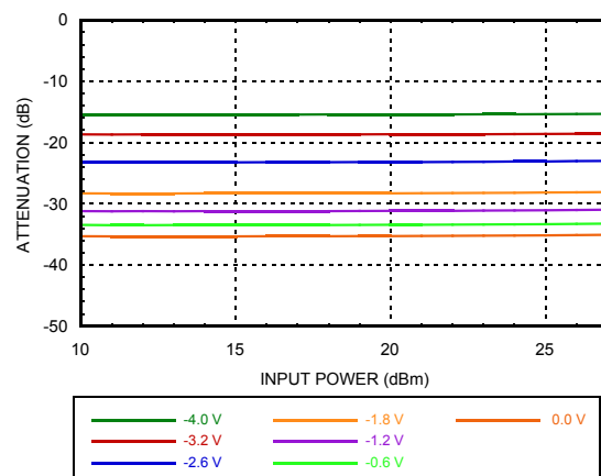
Attenuation vs. Pin @ 20 GHz over Vctrl2 Vctrl2 = Variable, Vctrl1 = 0V
