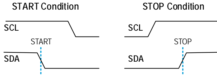
Figure 14. START and STOP Condition Waveform
