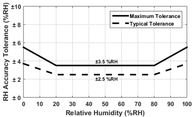
Figure 5. HS3003 RH Accuracy Tolerance at 25°C
