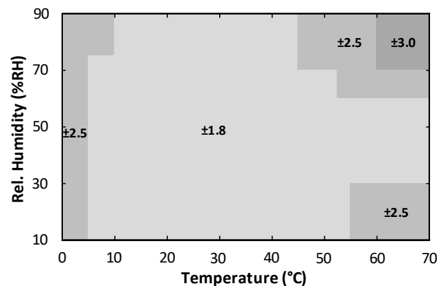
Figure 5. HS3002-MC1 RH Accuracy over Temperature
