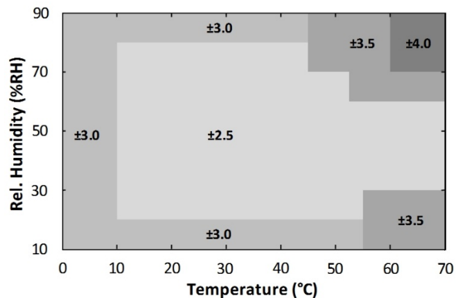
Figure 7. HS3003-MC1 RH Accuracy over Temperature
