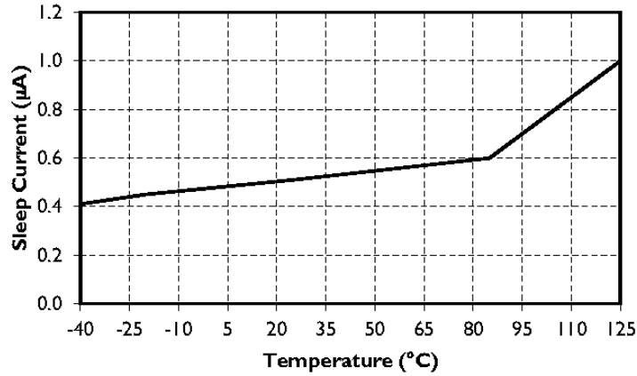
Figure 1. Sleep Current Variation over Temperature, V DD at 3.3V
