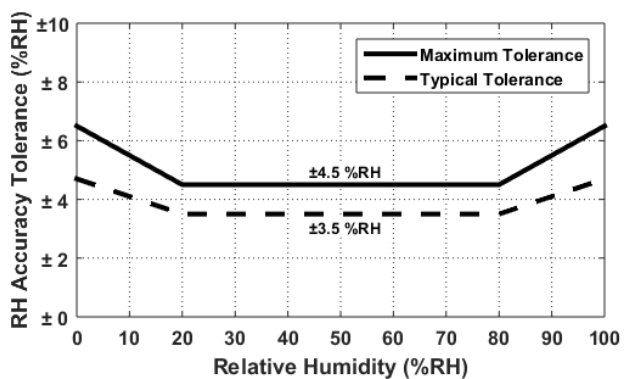
Figure 8. HS3004-MC1 RH Accuracy Tolerance at 25°C
