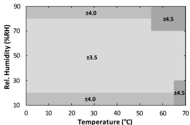
Figure 9. HS3004-MC1 RH Accuracy over Temperature
