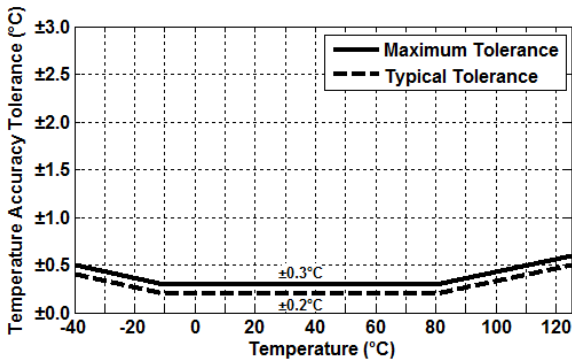
Figure 10. HS3001-MC1/HS3002-MC1 Temperature Sensor Accuracy Tolerance
