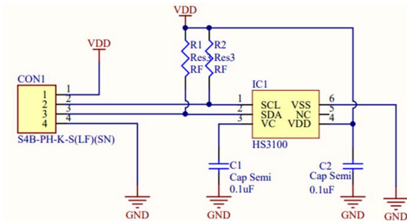
Figure 19. HS300x-MC1 Application Circuit
