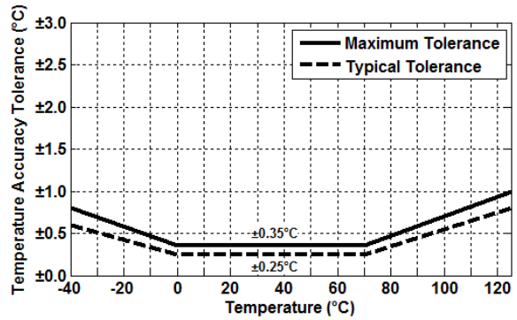
Figure 8. HS3003 Temperature Sensor Accuracy Tolerance
