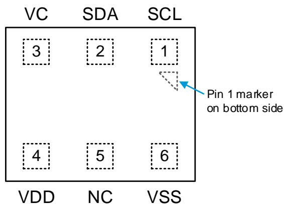
Figure 1. Pin Assignments for 3mm x 2.41mm 6-LGA Package – Top View
