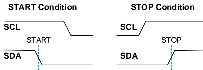
Figure 10. START and STOP Condition Waveform
