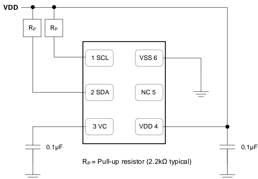
Figure 15. HS300x Application Circuit
