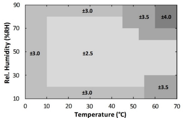
Figure 6. HS3003 RH Accuracy over Temperature
