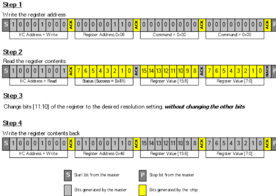
Figure 14. Sequence of Commands to Change the Relative Humidity Resolution
