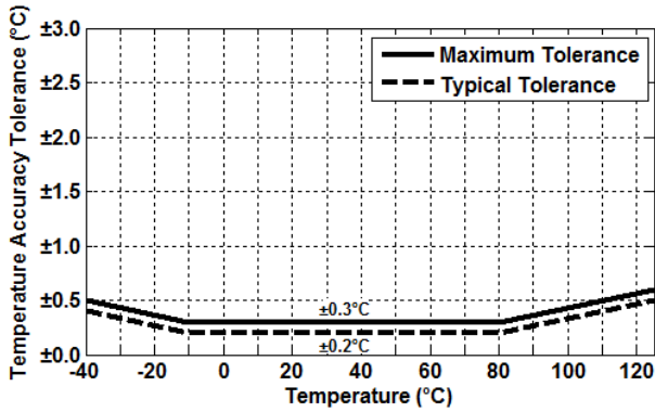
Figure 7. HS3001 Temperature Sensor Accuracy Tolerance
