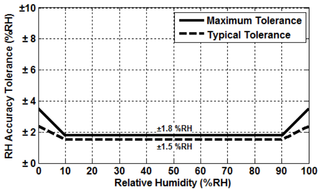
Figure 3. HS3001 RH Accuracy Tolerance at 25°C
