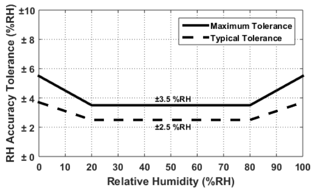
Figure 5. HS3003 RH Accuracy Tolerance at 25°C
