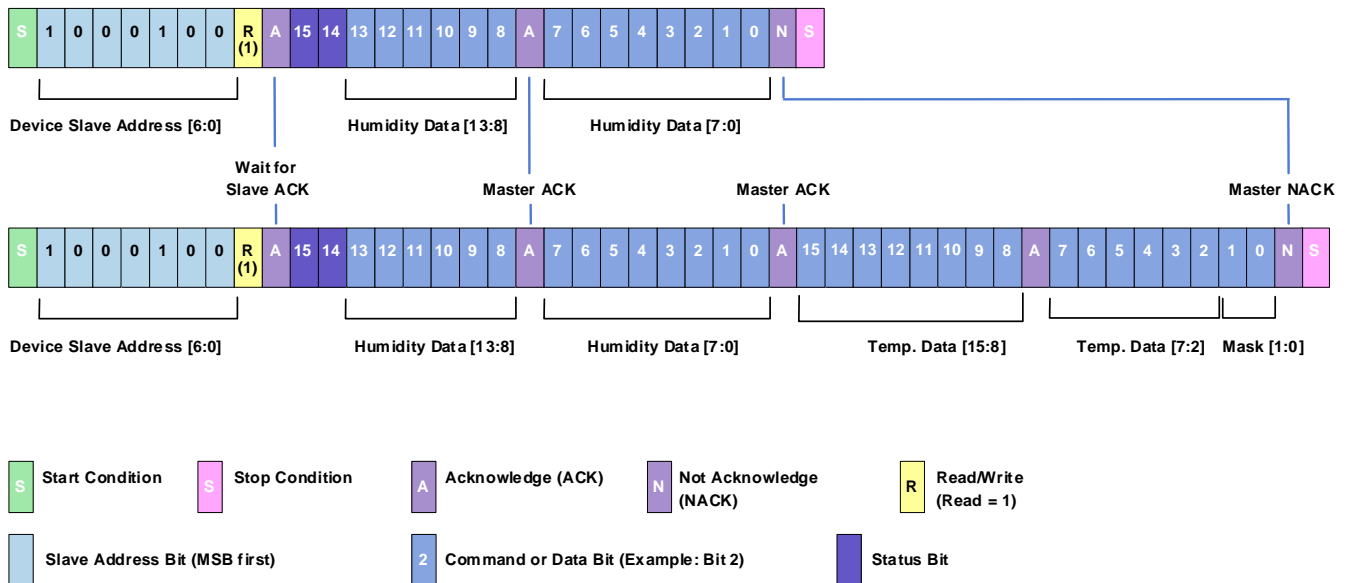
Figure 12. Data Fetch
