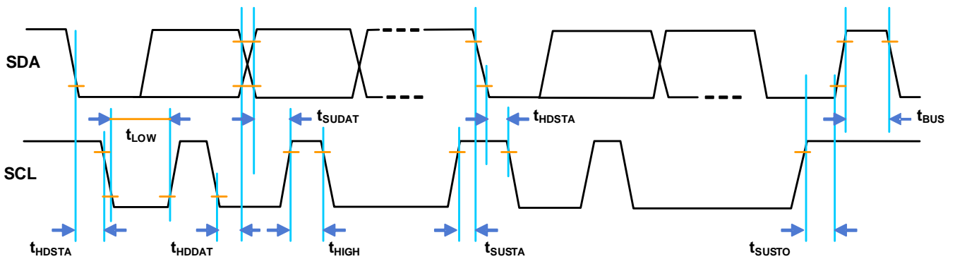
Figure 9. Timing Diagram
