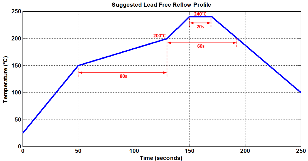
Figure 16. Recommended Soldering Profile
