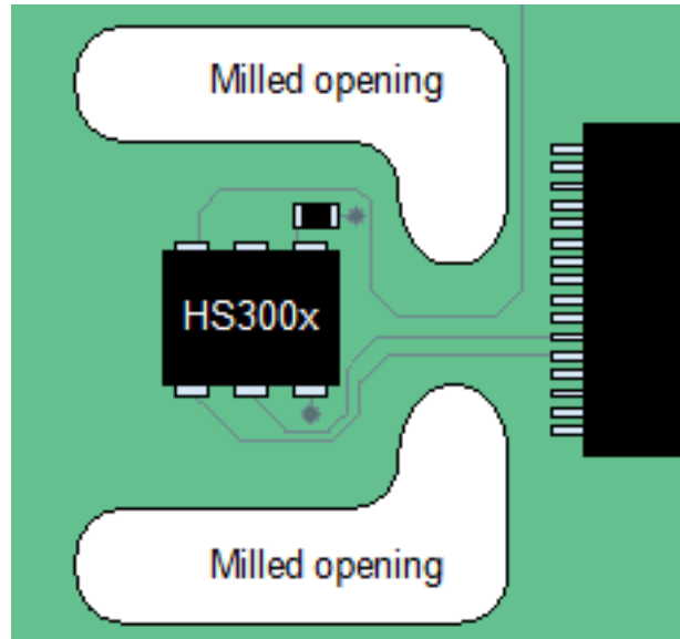
Figure 17. Milled PCB Openings for Thermal Isolation
