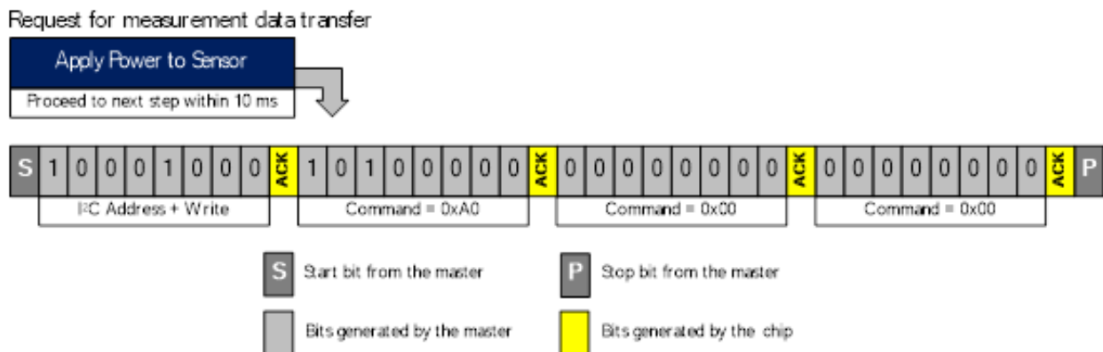
Figure 14. Sequence of Commands to Enter Programming Mode
