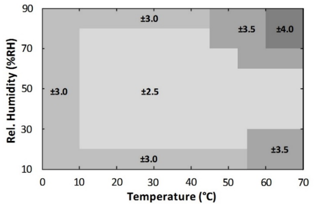
Figure 4. HS4013 RH Accuracy over Temperature
