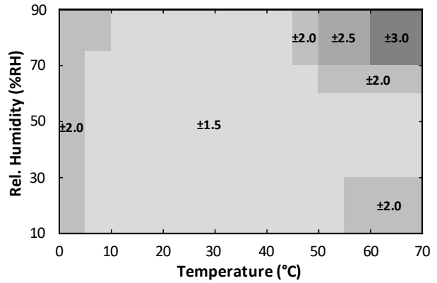
Figure 2. HS4011 RH Accuracy over Temperature
