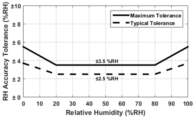
Figure 3. HS4103 RH Accuracy Tolerance at 25°C
