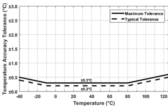
Figure 5. HS4111 Temperature Sensor Accuracy Tolerance
