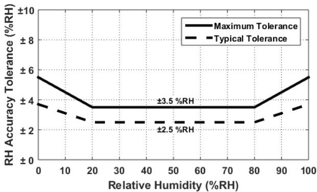
Figure 5. HS4113 RH Accuracy Tolerance at 25°C
