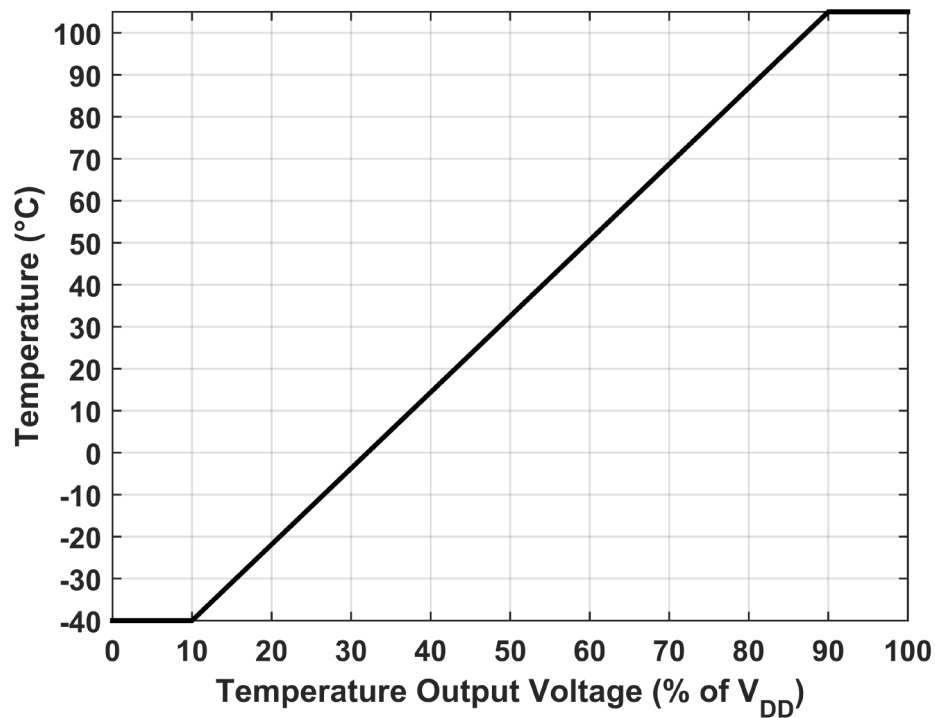
Figure 14. Temperature vs. VT Output Analog Voltage
