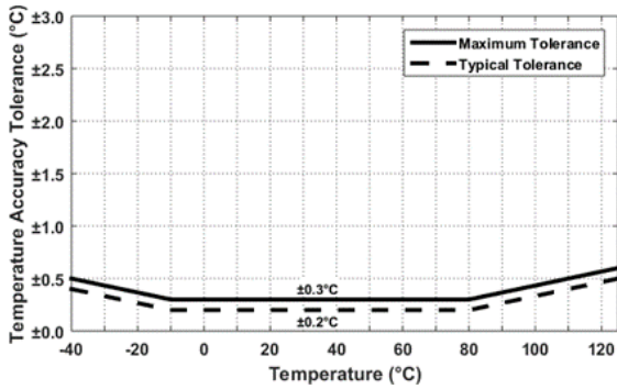
Figure 9. HS4111/HS4112 Temperature Sensor Accuracy Tolerance
