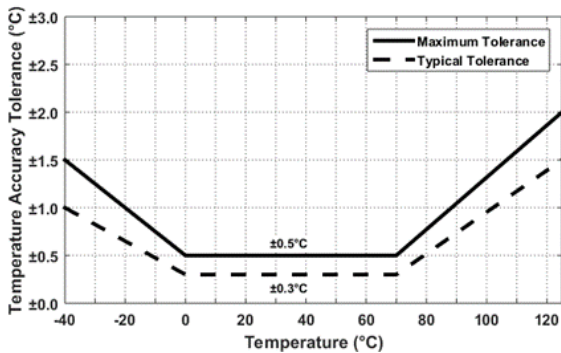
Figure 11. HS4114 Temperature Sensor Accuracy Tolerance
