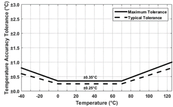
Figure 10. HS4113 Temperature Sensor Accuracy Tolerance
