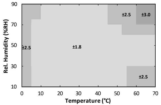
Figure 4. HS4112 RH Accuracy over Temperature
