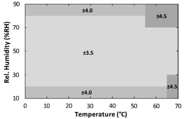
Figure 8. HS4114 RH Accuracy over Temperature
