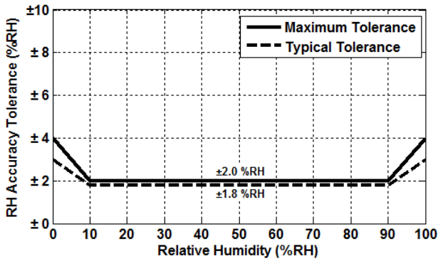
Figure 3. HS4112 RH Accuracy Tolerance at 25°C
