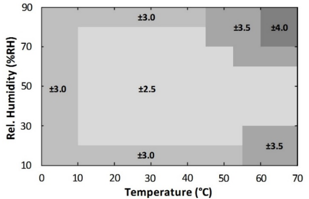
Figure 6. HS4113 RH Accuracy over Temperature
