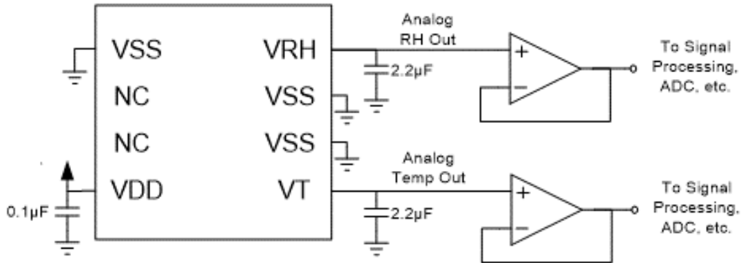
Figure 12. HS411x Application Circuit
