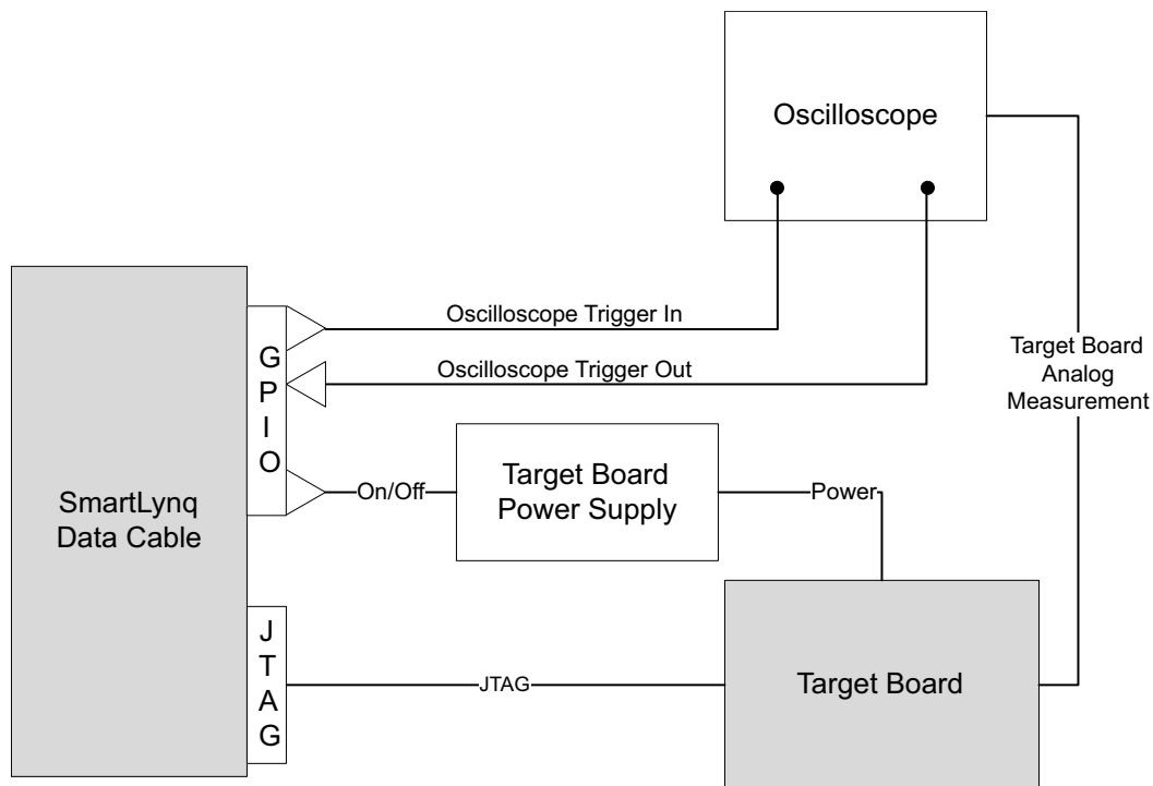
Figure 1-12: Sample Setup—Cable H to an Oscilloscope
