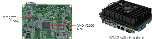
IB952 with Heatsink
