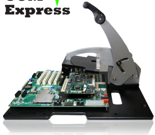
Open position
