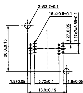
SOP IC51-0162-271-1 (16 Pins)
