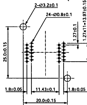
SOP IC51-0242-980 (24 Pins)
