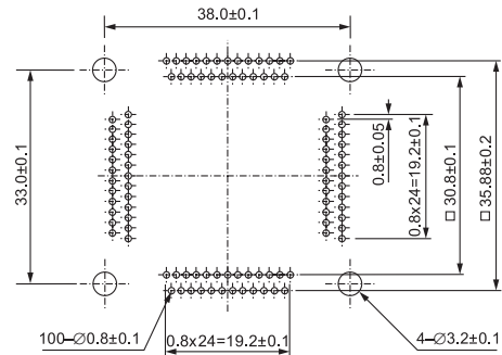
IC51-1124-1036-2 (112 Pins)
