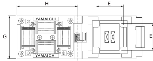
Outline Clamshell Socket Dimensions
