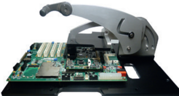
Closed position
