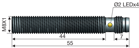
Fig. 12 Long body, flush version, plug
