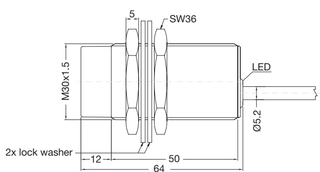
Fig. 34 Long body, non-flush version, cable
