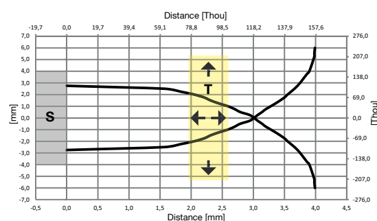
Fig. 4 Non-flush, 4mm
