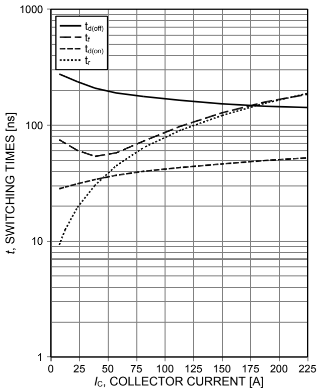
Figure 7. Typical switching times as a function of collector current (ind. load, T j =150°C, V CE =400V, V GE =0/15V, R G(on) =16Ω, R G(off) =6Ω, test circuit in Fig. E)
