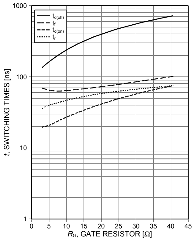
Figure 8. Typical switching times as a function of gate resistor (ind. load, T j =150°C, V CE =400V, V GE =0/15V, I C =75A, test circuit in Fig. E)
