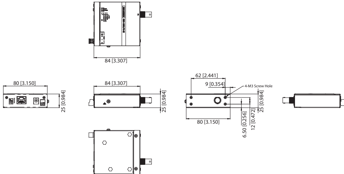
Panel Cut-out Dimensions (W x H x D): 84 x 80 x 25 mm (3.307 x 3.15 x 0.984 in.)
