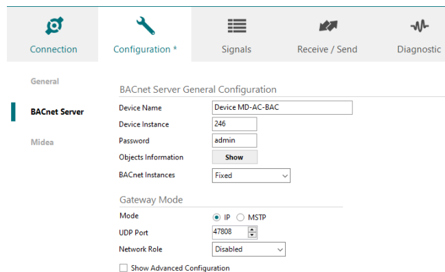
Figure 7.3 Intesis MAPS BACnet configuration tab
