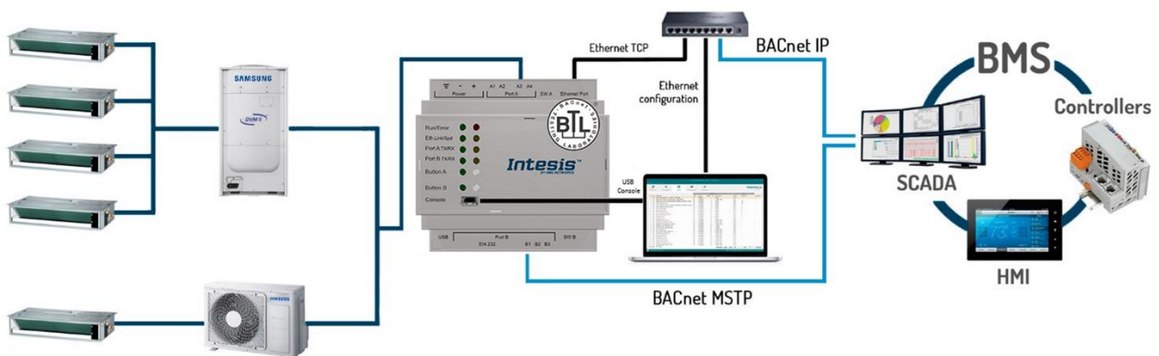
Integration of Samsung NASA AC compatible systems into BACnet/IP or BACnet MSTP control systems
