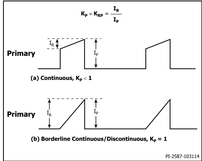
Figure 21. Continuous Mode Current Waveform, K_p \leq 1 .
