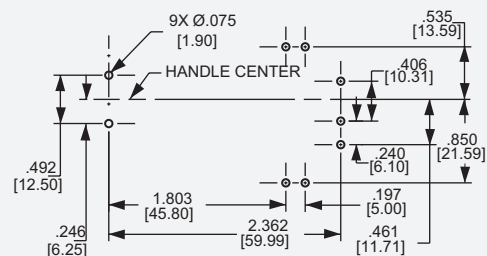
Mounting Detail
