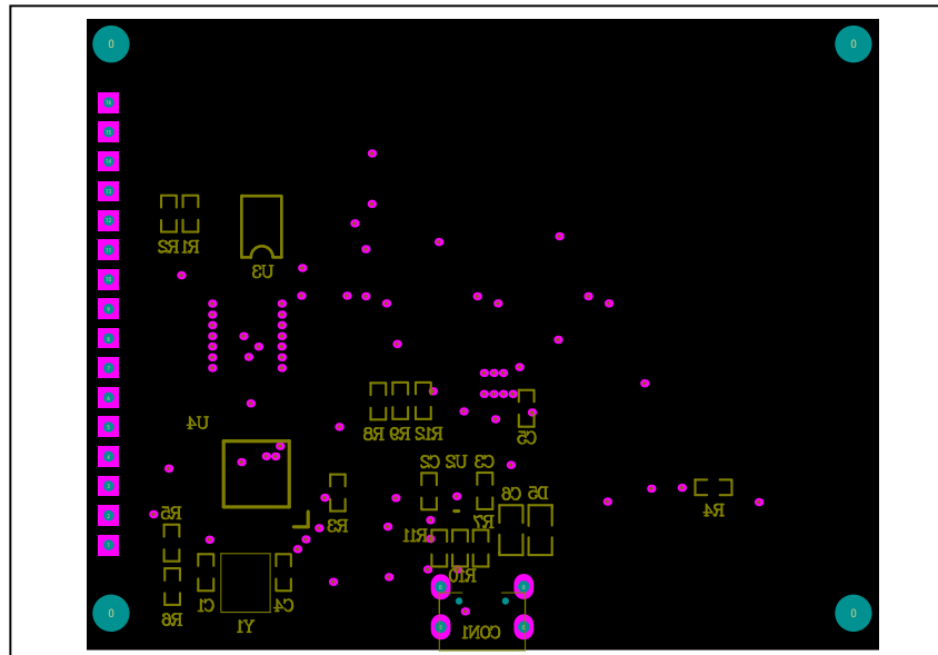
Figure 5: Board Component Placement Guide - Bottom Layer
