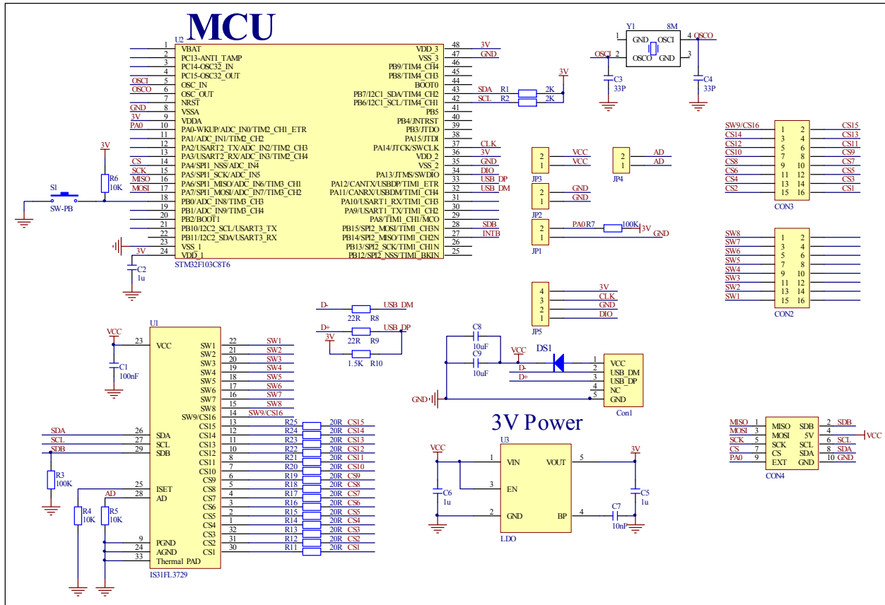
Figure 3: IS31FL3729 Application Schematic
