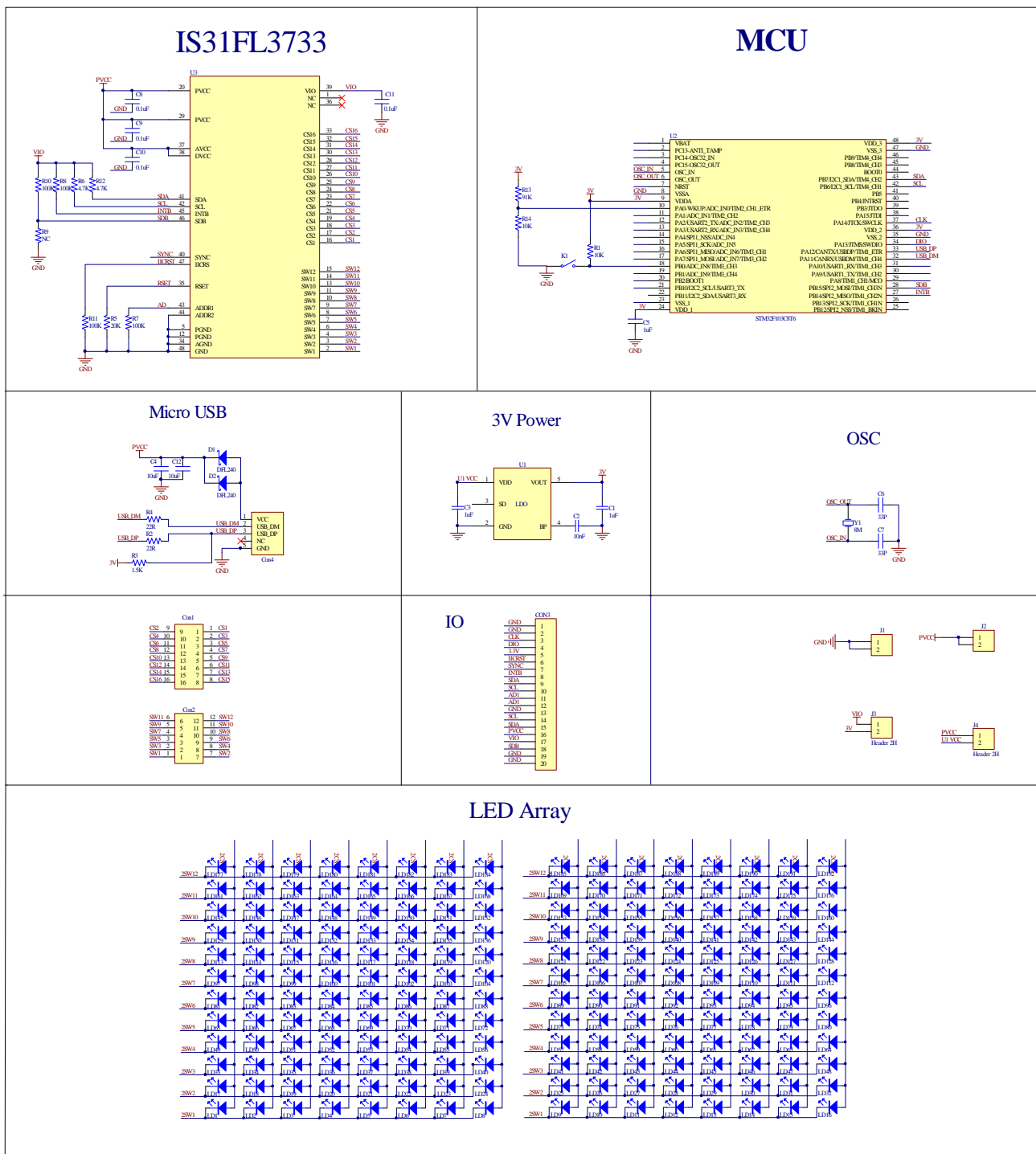
Figure 2: IS31FL3733 Application Schematic
