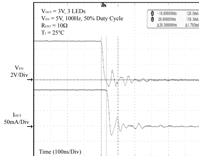
Figure 36 V_{EN} vs. I_{OUT} Delay and Falling Edge
