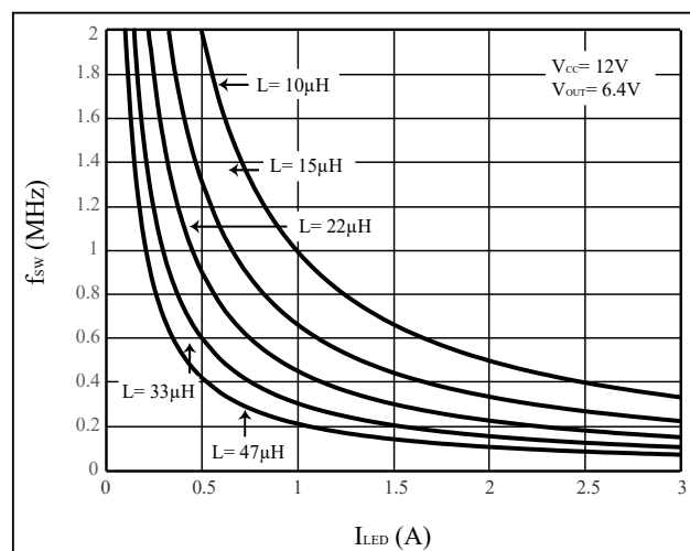
Figure 34 Inductance Selection Based On 30% Current Ripple
