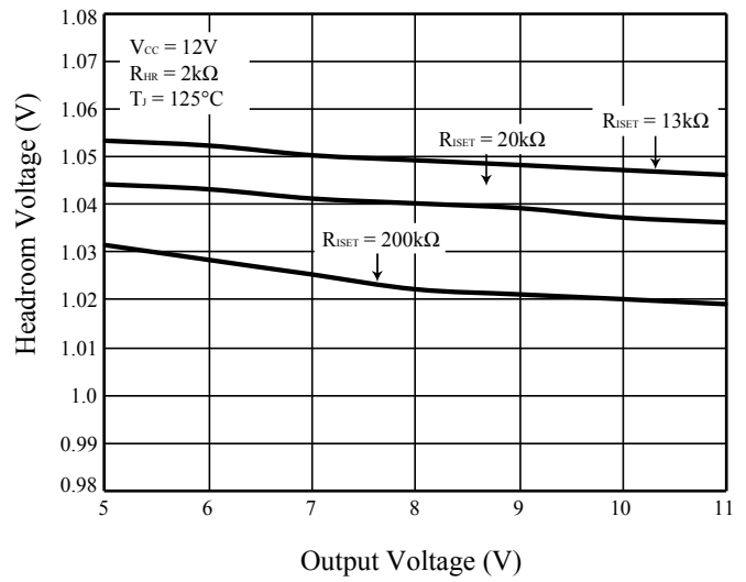
Figure 15 V_{HR} vs. V_{OUT}
