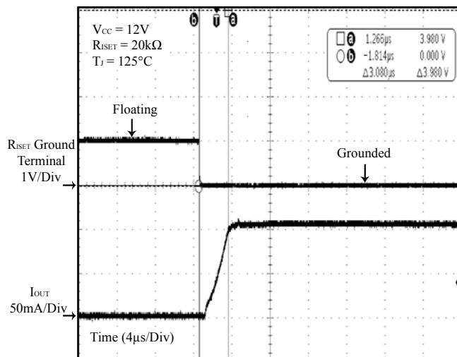
Figure 49 ISET PWM On Delay Time for IS32LT3124B/C/E/F
