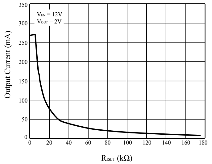
Figure 11 Output Current vs. R_{ISET}
