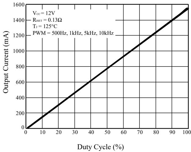
Figure 16 I_{OUT} vs. Duty Cycle
