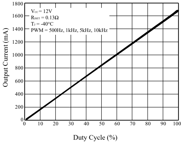
Figure 14 I_{OUT} vs. Duty Cycle
