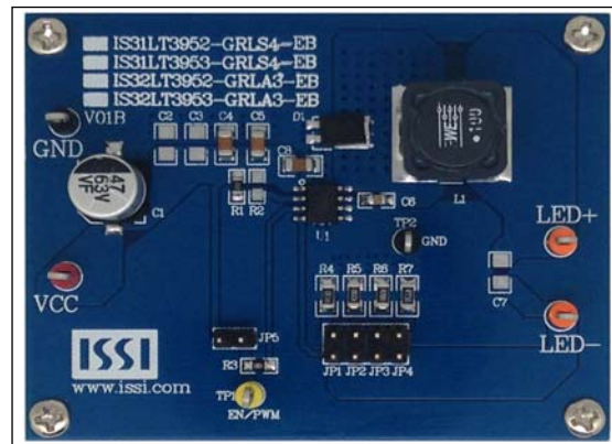
Figure 1: Photo of IS31LT3953_IS32LT3953 Evaluation Board
