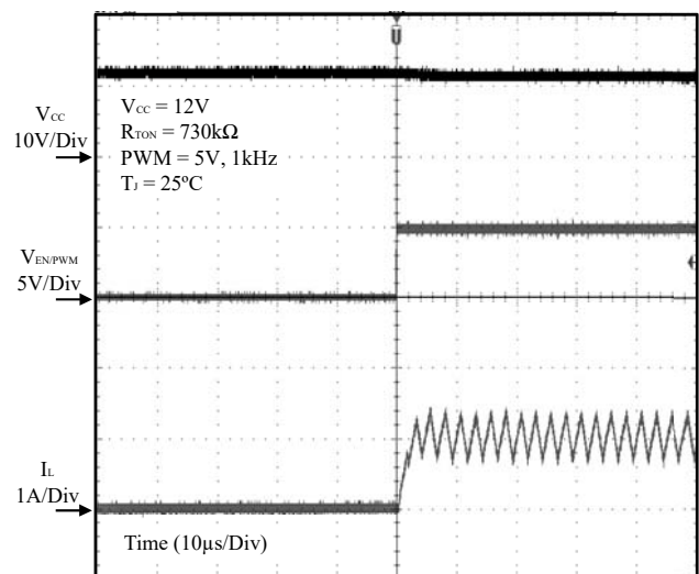
Figure 25 PWM On
