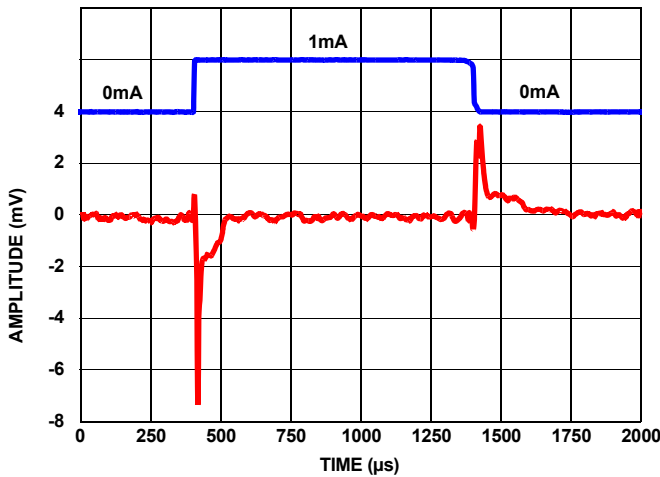
FIGURE 45. LOAD TRANSIENT RESPONSE AT 1mA LOAD AT 1μF
