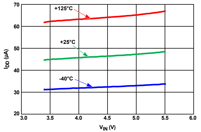
FIGURE 106. I_{IN} vs V_{IN} , OVER-TEMPERATURE
