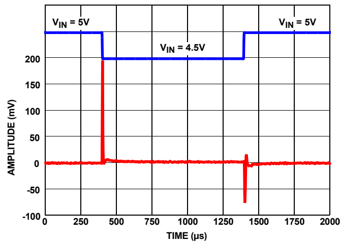
FIGURE 126. LINE TRANSIENT RESPONSE WITH 0.1\mu F LOAD
