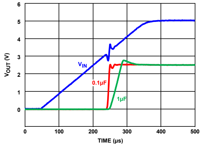
FIGURE 80. TURN-ON TIME
