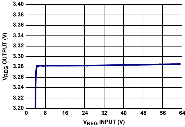
FIGURE 77. V REG OUTPUT vs INPUT VOLTAGE
