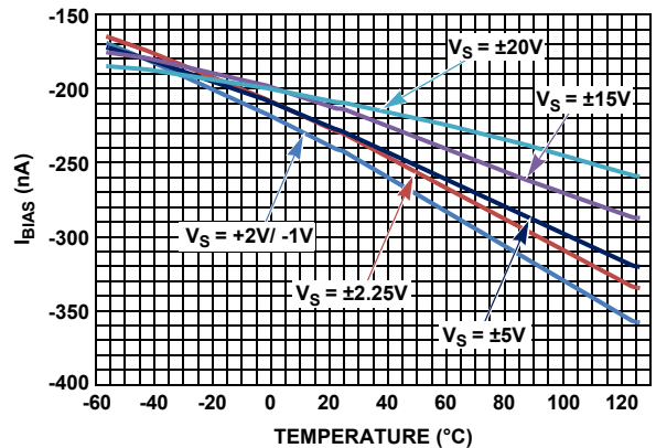
FIGURE 8. I_{BIAS} vs TEMPERATURE vs SUPPLY
