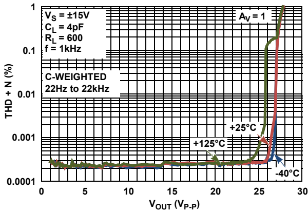
FIGURE 21. THD+N vs OUTPUT VOLTAGE ( V_{OUT} ) vs TEMPERATURE, A_V = 1 f = 1\text{kHz} , R_L = 600\Omega
