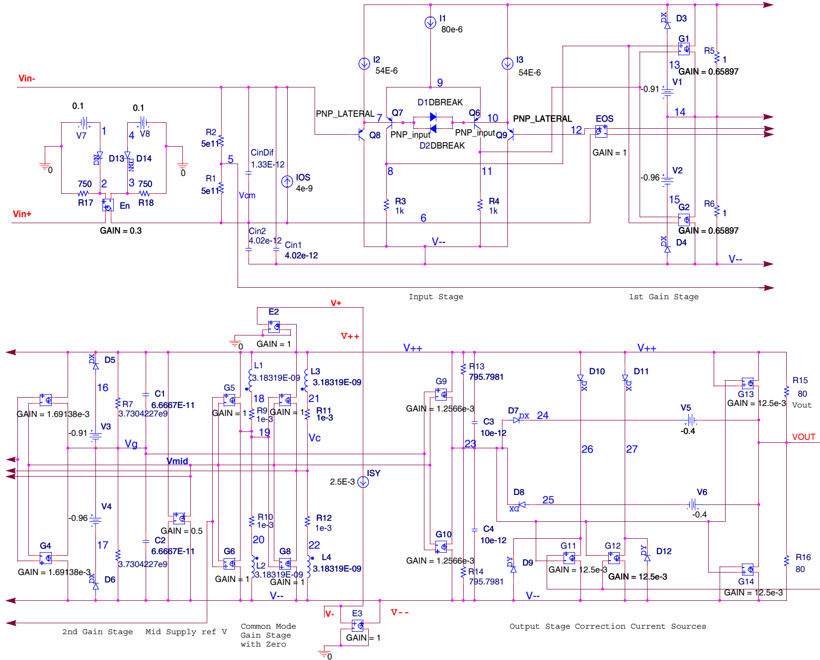
FIGURE 64. SPICE SCHEMATIC
