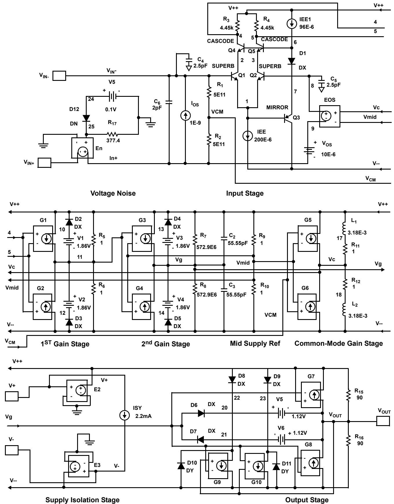
FIGURE 41. SPICE SCHEMATIC
