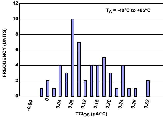
FIGURE 32. TC_{I_{OS}} HISTOGRAM
