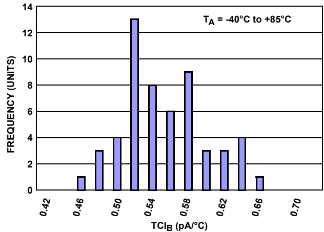
FIGURE 33. TC_{I_B} HISTOGRAM
